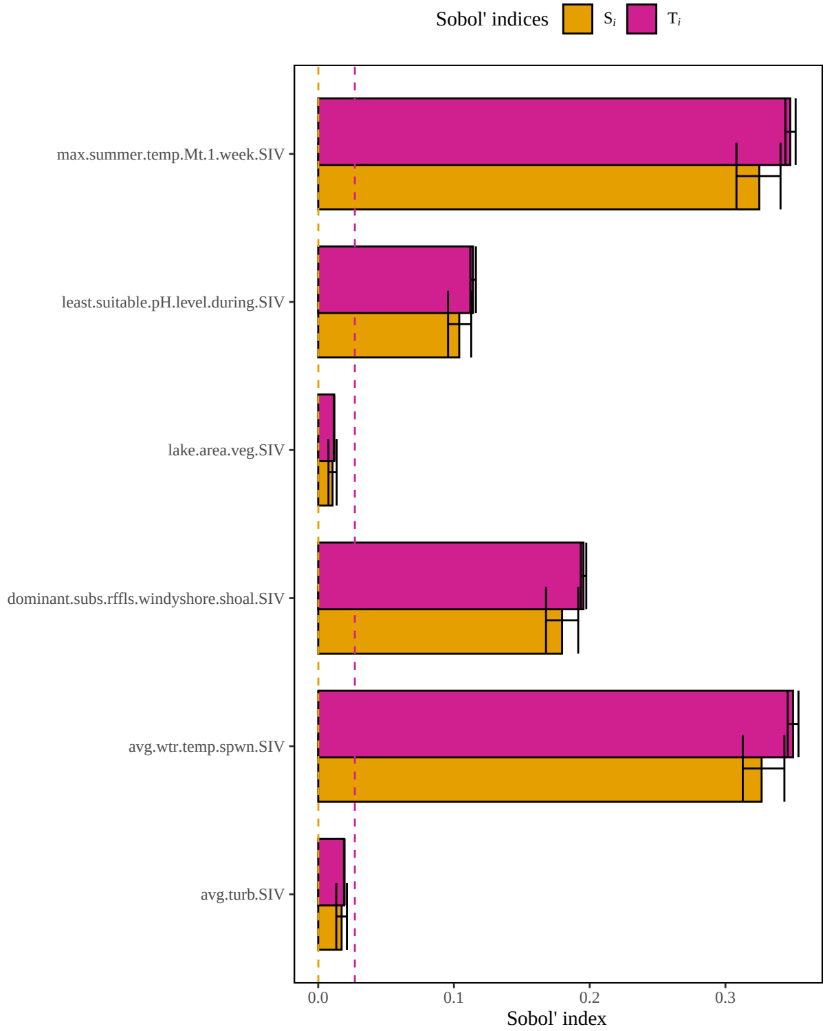
Figure 5. Results of a sensitivity analysis for the commonshinerLac model based on a geometric mean structure. Dashed lines represent baseline numerical approximation error for S_i and T_i ( i.e. , dummy variables).
