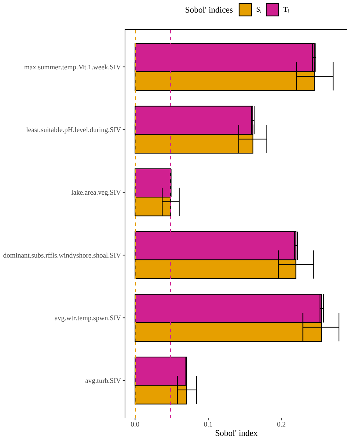
Figure 4. Results of a sensitivity analysis for the commonshinerLac model based on an arithmetic mean structure. Dashed lines represent baseline numerical approximation error for S_i and T_i ( i.e. , dummy variables).
