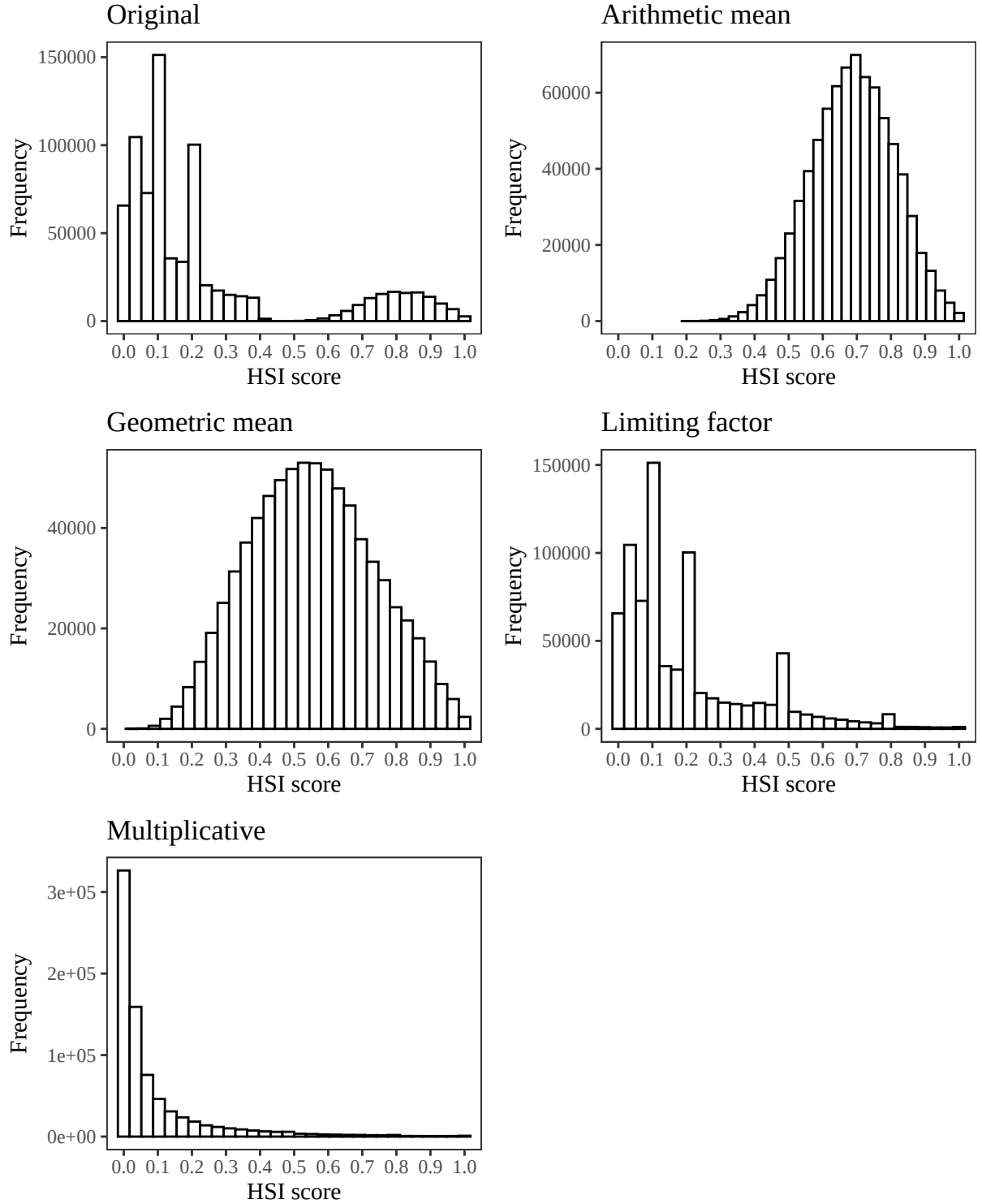
Figure 2. Empirical distributions of HSI scores for the commonshinerLac model using the original author-specified model equation from Trial et al. (1983), and an arithmetic mean, geometric mean, limiting factor, and multiplicative structure incorporating all SIV variables. Note differences in the y axis.
